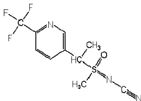
Fig.1 : Sulfoxaflor structure .
